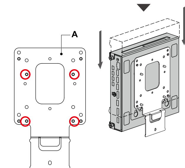
Position of a screw hole (four positions)
